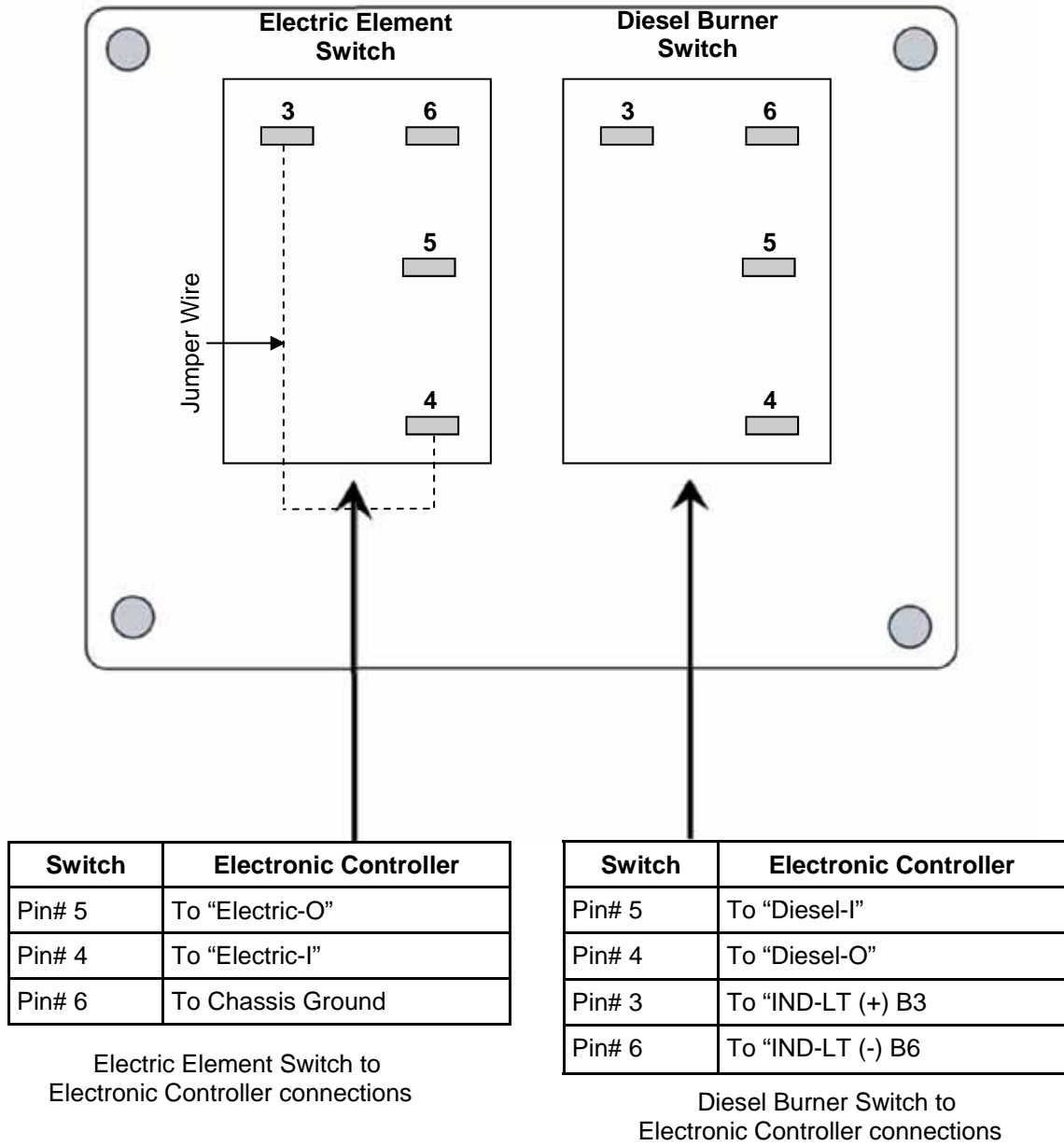
Aqua-Hot 400D Switch Panel, Rear View
