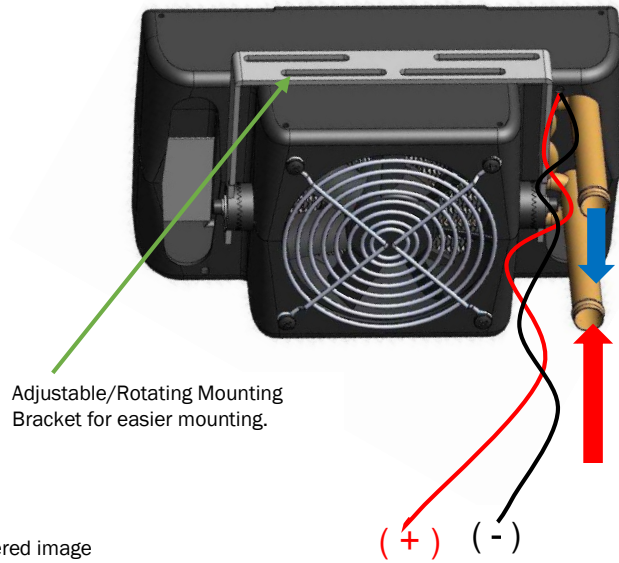
Figure 2: Back View
